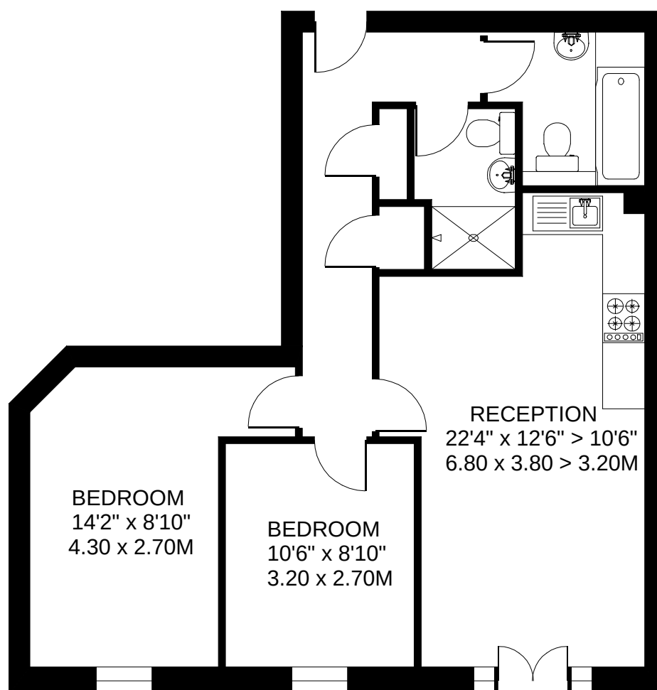
FIRST FLOOR
