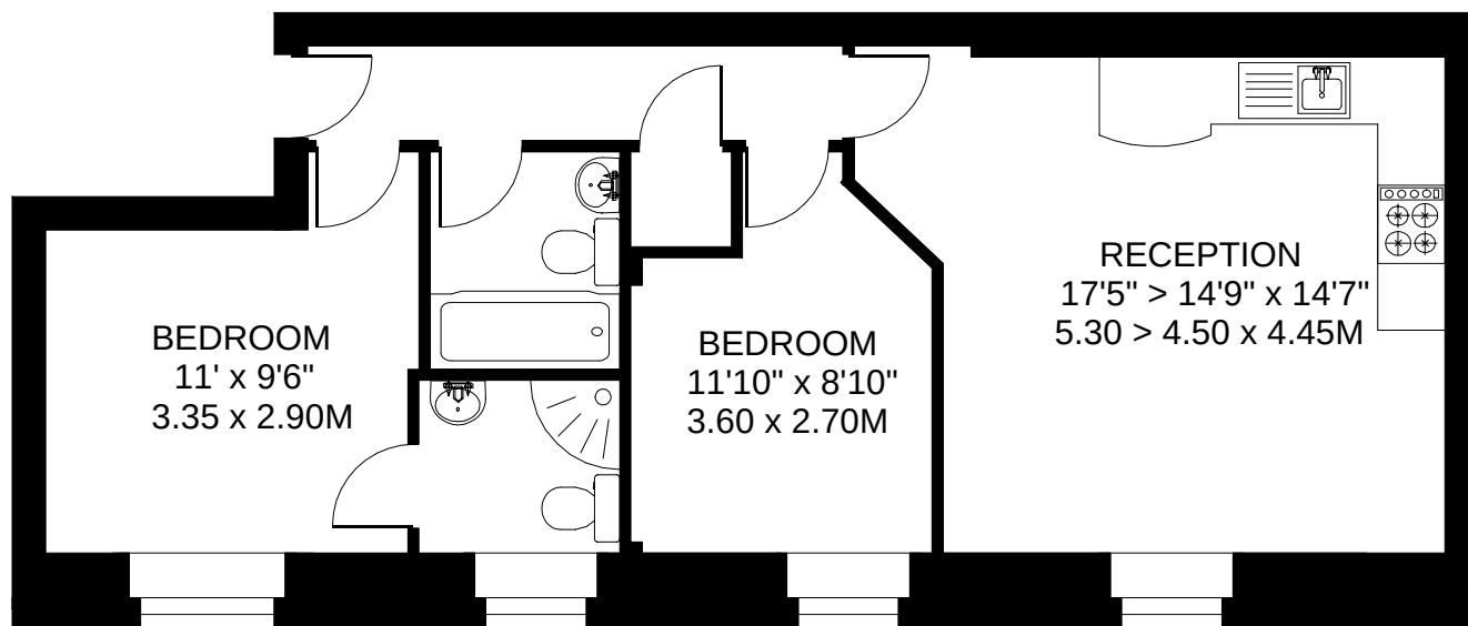
SECOND FLOOR
