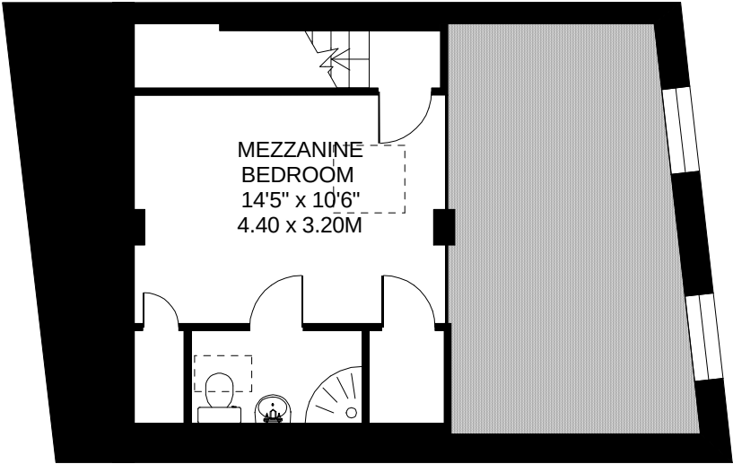
THIRD FLOOR
